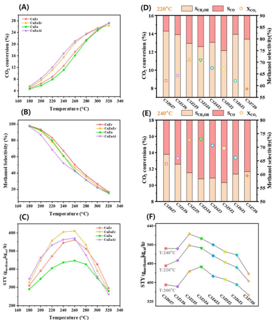
Fig. 1. Methanol formation and ^{13}\text{C} exchange over unmodified and oxide-modified Cu catalysts.
