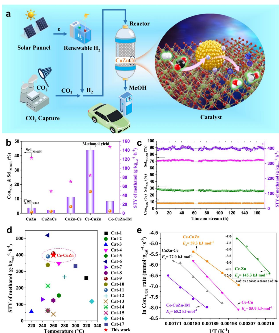
Fig. 1. CO 2 conversion, methanol selectivity, methanol yield, and catalyst stability over the Cu–oxide samples.
